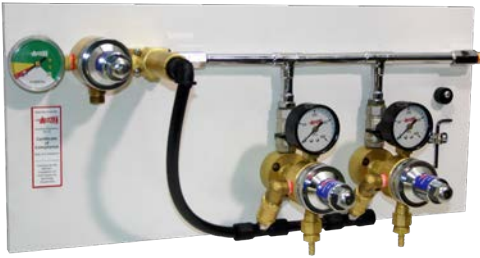
2 WAY ANDALE AS5034 GAS BOARD
